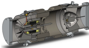
Cutaway of Fuel Flow Transmitter
